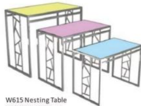
W615 Nesting Table 700x700xH750mm 800x800xH900mm 900x900xH1050mm 1200x650xH650mm 1300x650xH800mm 1400x650xH950mm
