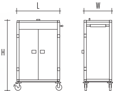
Terse M2 CXQ41A2 L770×W500×H1290mm L30.31"×W19.69"×H50.79"
